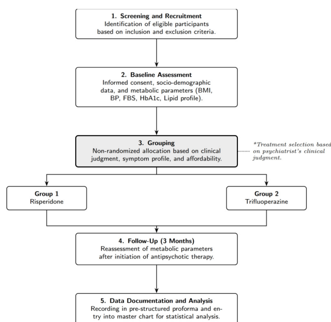
Figure 1: Study procedure
